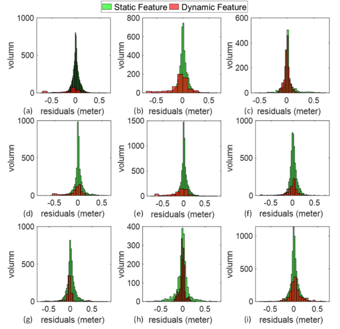
Fig. 17. Illustration of the residual distributions of the compared scenarios on a single epoch. The x-axis denotes the value of residuals. The y-axis represents the volume associated with each bin of the residuals in the histogram. The residual of the static feature is marked in green, while the residual of the dynamic feature is marked in brown. The residuals are presented under scenarios (a) 20% of dynamic objects; (b) 50% of dynamic objects; (c) 80% of dynamic objects; (d) D2 value equals 0.00357; (e) D2 value equals 0.00630; (f) D2 value equals to 0.00846; (g) right side dynamic objects with relative speed 5 m/s; (h) both side dynamic objects with relative speed 10 m/s; (i) both side dynamic objects with relative speed 20 m/s.
