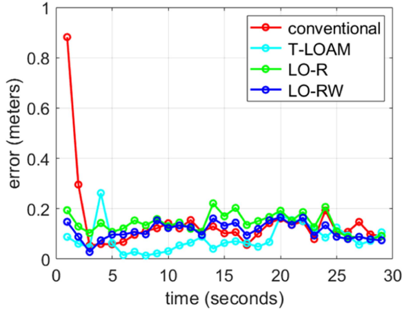
Fig. 18. Positioning error of the four methods. The x-axis and y-axis denote the epoch and error, respectively.
