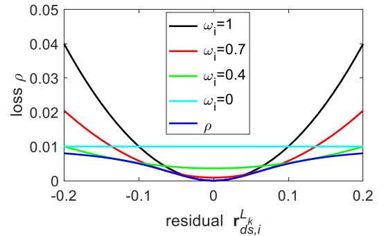
Fig. 6. \rho(\ast) with respect to different \omega_i if k = 0.1 . \hat{\rho} represents the optimal loss.
