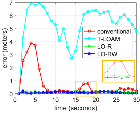
Fig. 20. Positioning error of the four methods in the high-dynamic scene. The x-axis and y-axis denote the epoch and error, respectively. The orange box is the area with dynamic and static objects.
