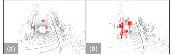
Fig. 10. Illustration of the simulated point cloud with different percentages of dynamic objects: (a) 10% dynamic objects; (b) 60% dynamic objects.
