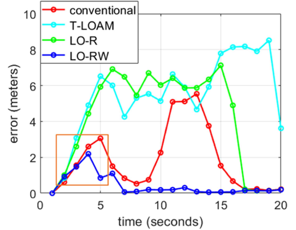
Fig. 23. 3D Positioning error of the four methods in nuScenes . The x-axis and y-axis denote the epoch and error, respectively. The orange box is the tunnel-like area (see Fig. 22(a)) with dynamic and static objects. It has a negative impact on state estimation.
