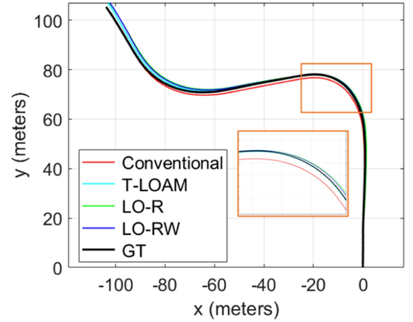
Fig. 19. 2D positioning trajectories of the four methods. The x-axis and y-axis denote the x and y directions, respectively. The black curve represents the ground truth.
