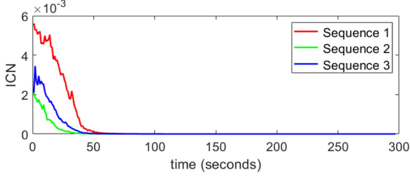
Fig. 16. Illustration of the ICN from \mathbf{J}_d^T \mathbf{J}_d with different geometric distributions of dynamic points.
