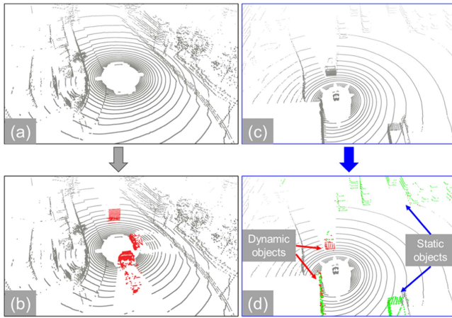
Fig. 1. Illustration of the contributions of this work. LiDAR points in a 3D static environment are marked in grey. (a) Represent the scanned cloud in the static environment; (b) the red cloud represents the dynamic vehicles produced by the proposed vehicle simulator. It is integrated with (a) for investigating the impacts of dynamic objects on the degeneration of LiDAR odometry; (c) the grey cloud represents the simulated point cloud with dynamic objects (d) the proposed joint weighting optimization for LiDAR odometry with dynamic object awareness. There are both healthy features and ill features on static or dynamic objects simulated based on (b). Healthy ones assigned with high weight are marked in green. The unhealthy ones assigned with low weights are marked in red.
