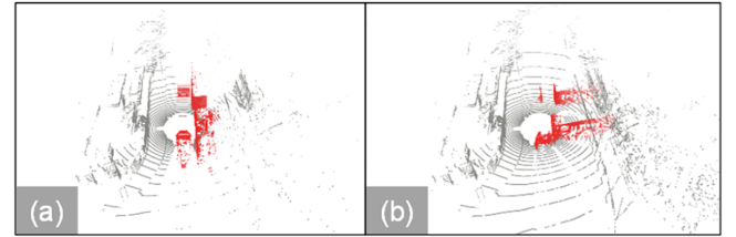
Fig. 11. Illustration of the simulated point cloud (a) and (b) with vertical and horizontal dynamic points distribution.
