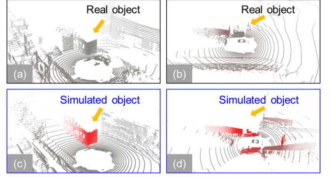
Fig. 5. Illustration of the simulated point cloud (c) and (d) that contained objects that matched the real data in (a) and (b).
