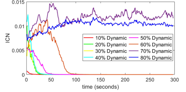
Fig. 15. Illustration of the inverse condition number (ICN) from \mathbf{J}_d^T \mathbf{J}_d with different levels of dynamic points.
