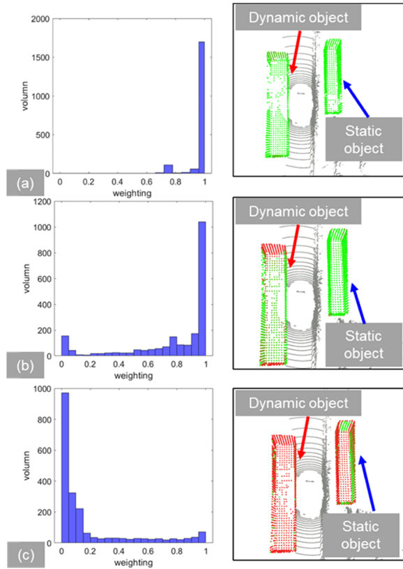
Fig. 25. Illustration of weighting by different penalty parameters of state optimization. (a) Penalty parameter k = 1 ; (b) penalty parameter k = 0.1 ; (c) penalty parameter k = 0.01 ; the lower weighting is indicated by red while higher weighting is marked by green.
