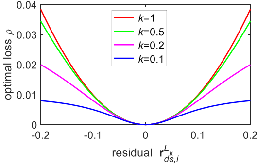
Fig. 7. Optimal \hat{\rho} with respect to different k .
