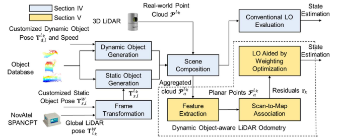
Fig. 2. Overview of the proposed method.
