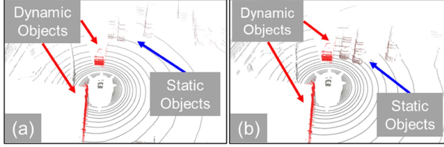
Fig. 14. Illustration of the integrated point cloud with dynamic objects for evaluation in nuScenes (the data contains parked bus). (a) the scanned point cloud at timestamp t ; (b) the scanned point cloud at timestamp t + 1 .
